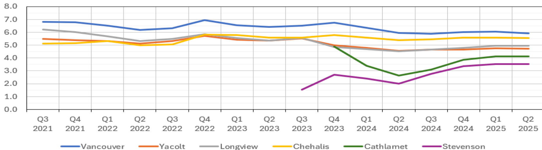
PM 2.5 - rolling annual averages - µg/m 3 [excluding flagged wildfire days] National Standard - 9 µg/m 3 (3-year annual average)
